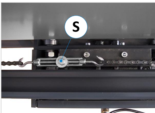
Figure 13: Fitting and tensioning the link chain
