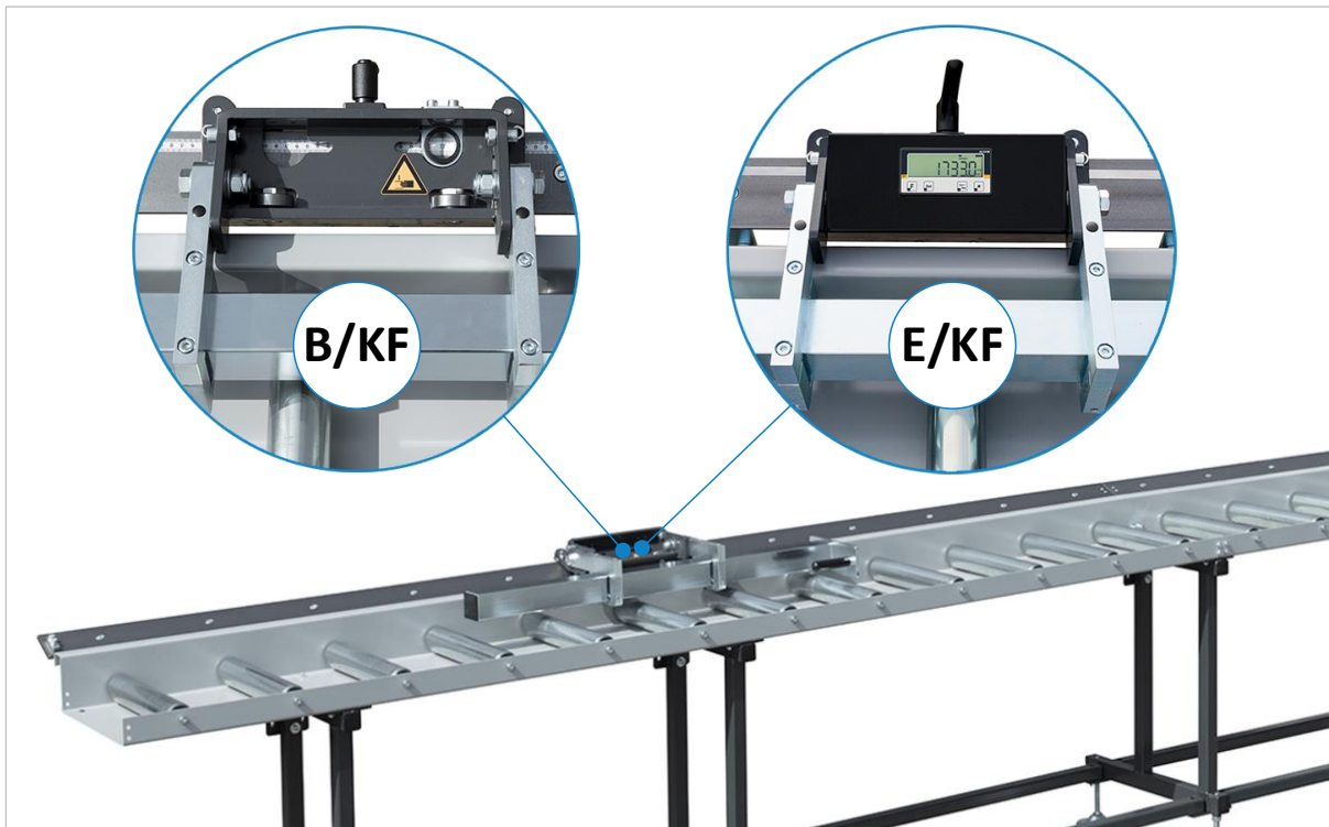
Figure 4: Roller and measuring conveyors EXAKT STANDARD B/KF and E/KF
