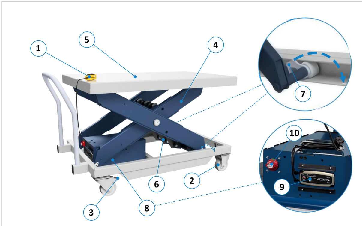
Figure 4: Components and controls of HS 2000 | AH
