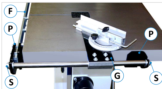
Figure 45: Mitre fence “Top”
