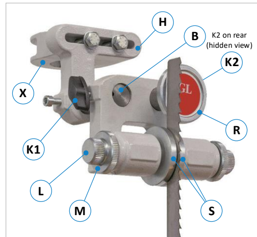
Figure 29: GL 456 - Structure and components
