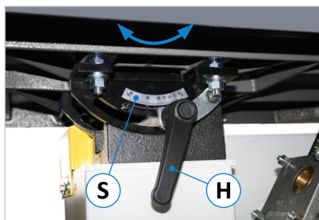
Figure 28: Adjust table inclination
