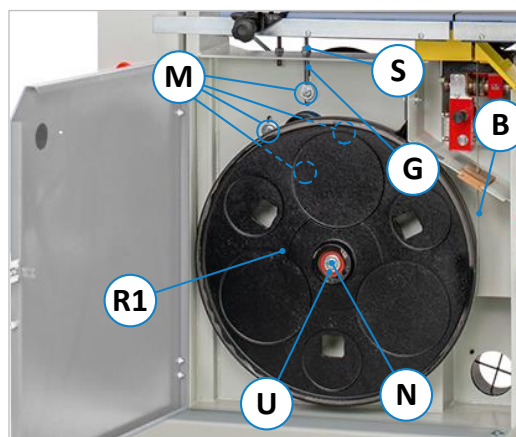
Figure 57: Replacing the V-belt(s)
