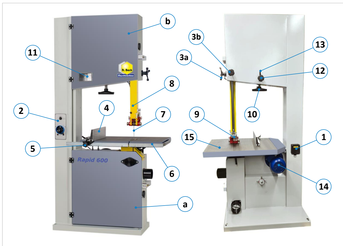
Figure 15: Components and controls
