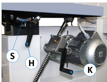
Figure 44: Adjust the table Inclination
