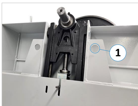
Figure 8: Crane eyelet
