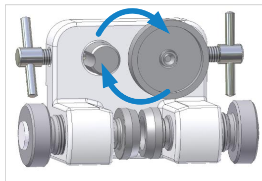
Figure 41: Convert top guide to left
