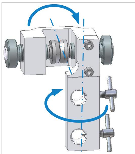
Figure 40: Convert bottom guide to left
