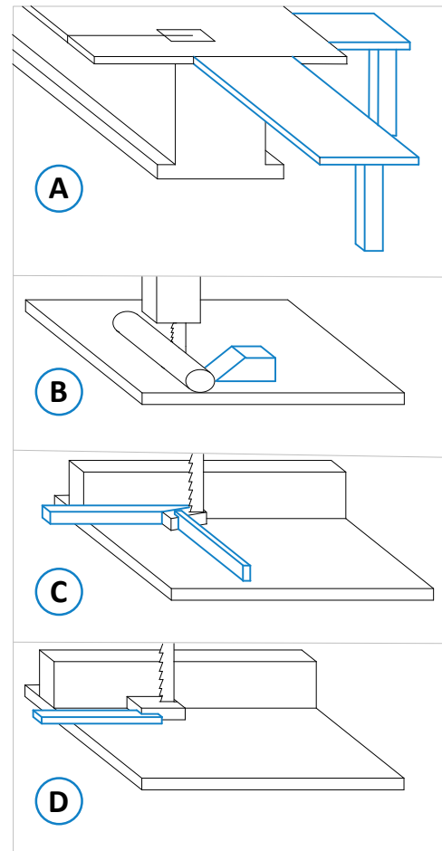
Figure 36: Table extensions and tools
