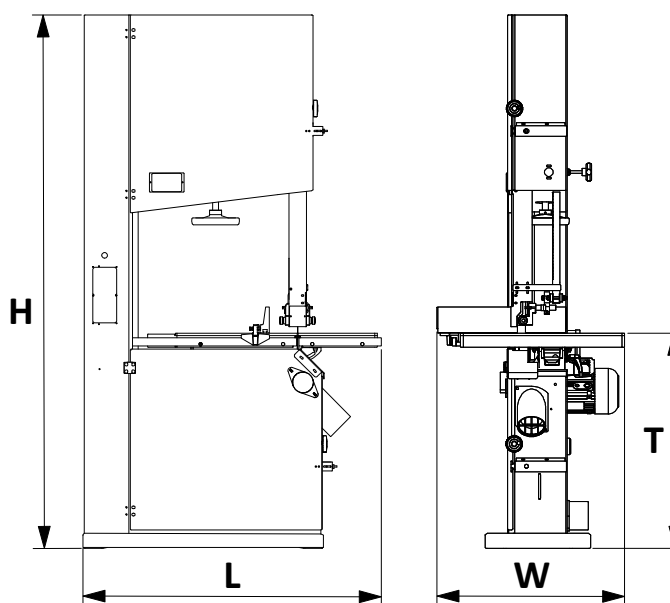
Figure 6: Dimensions
