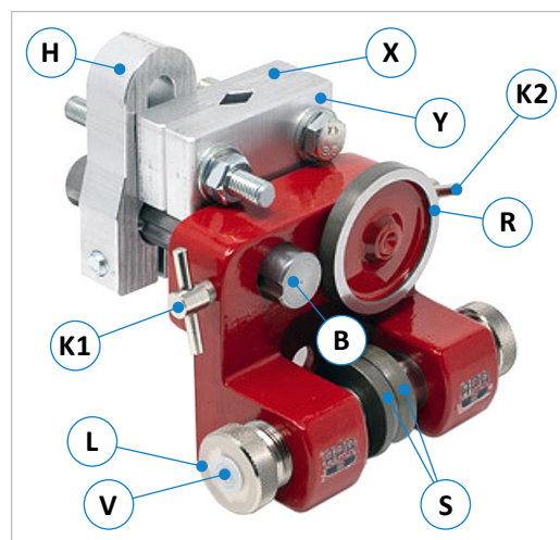
Figure 37: APA - Structure and components
