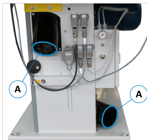
Figure 26 : raccords d'aspiration
