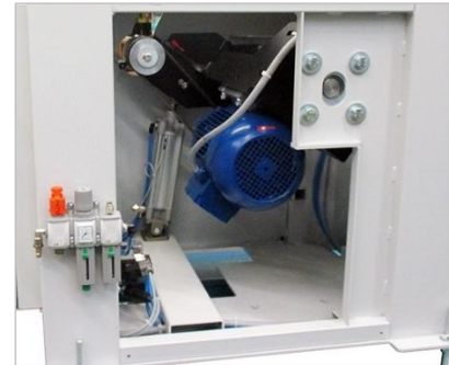
Figure 49: motor cover plate removed
