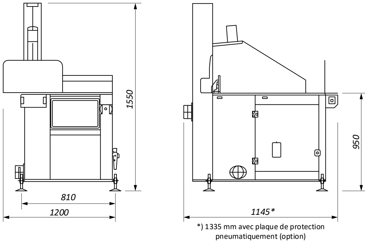
Figure 10 : dimensions UTK 500
