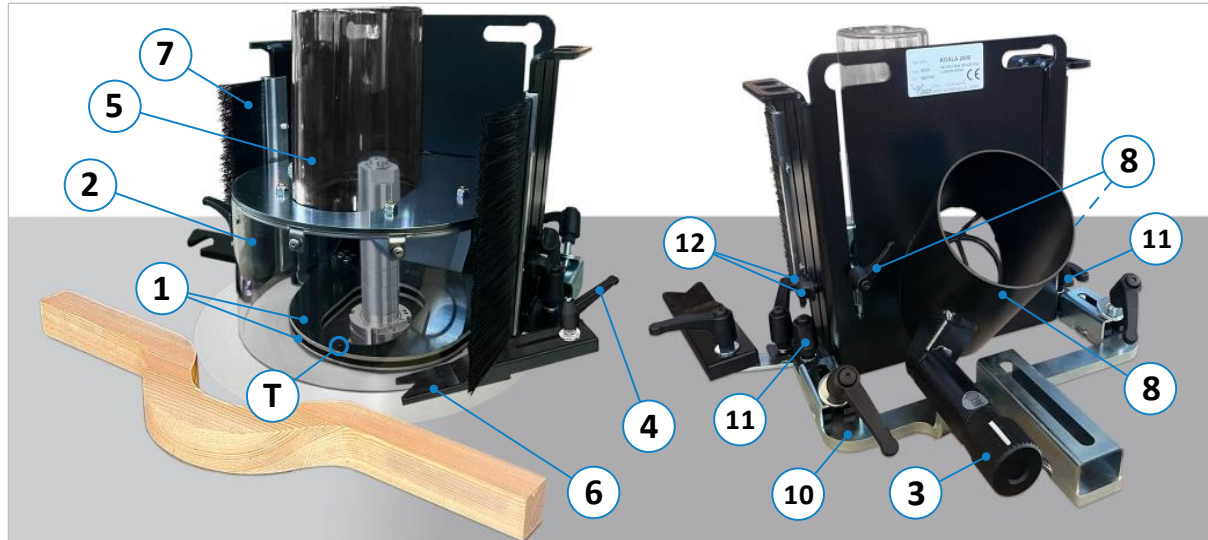
Figure 7: Operating elements of the KOALA 1637 ring fence
