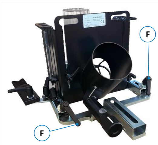
Figure 6: Attaching the protective device
