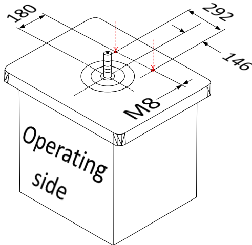
Figure 5: Drill and tap threaded holes
