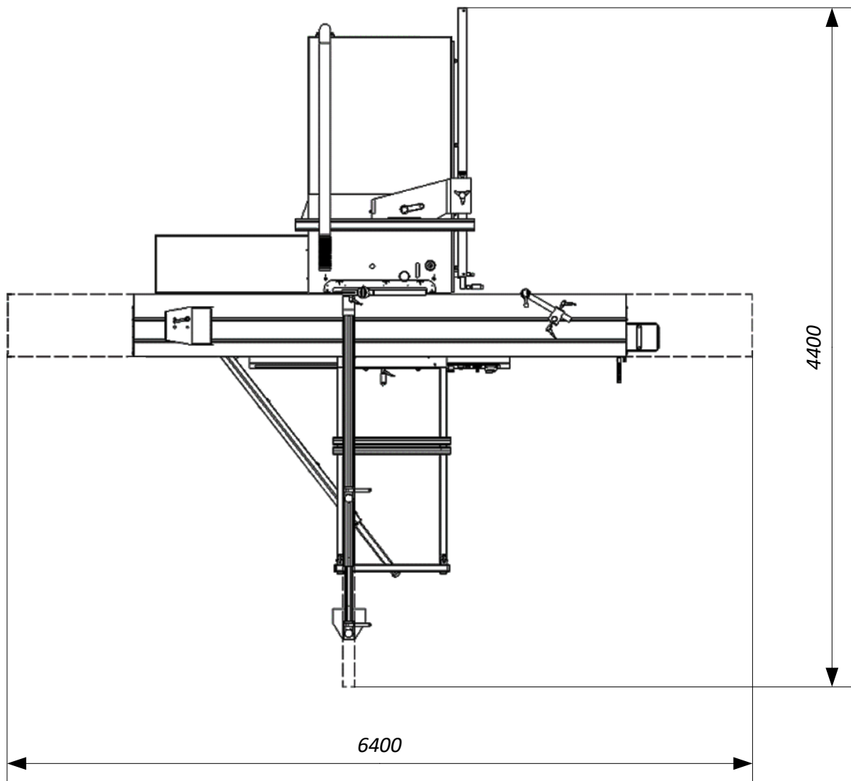
Figure 8: Maximum dimensions - top view
