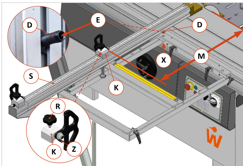
Figure 41: Check and readjust the tape measure
