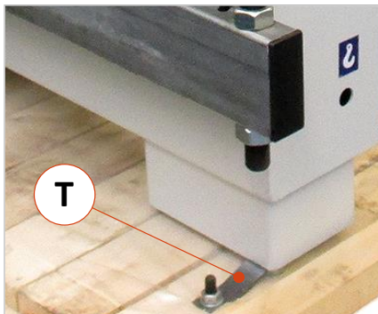
Figure 12: Transport shackle (4 x)
