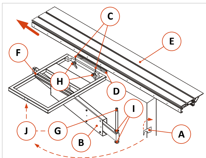
Figure 37: Mounting and adjusting the cross-cut carriage
