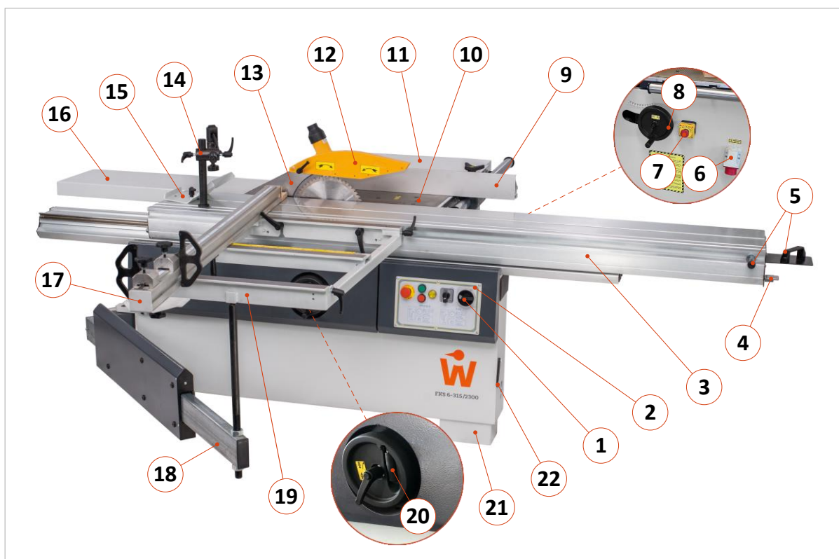
Figure 16: Components and controls
