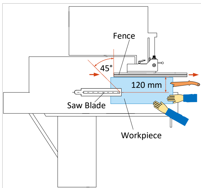
Figure 4: Cutting short workpieces to width
