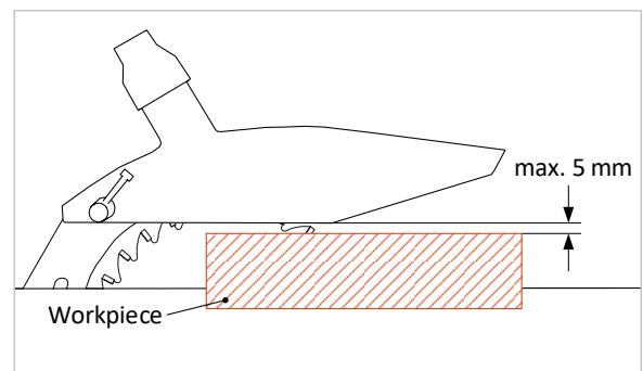
Figure 32: Adjusting the saw blade guard
