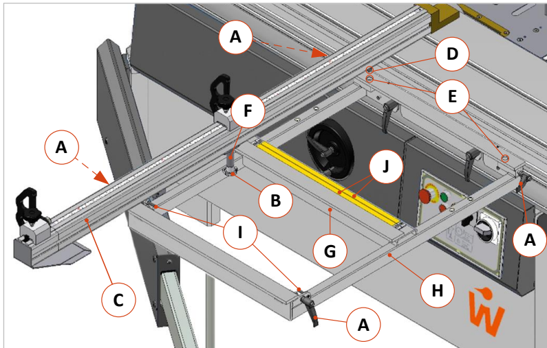
Figure 38: Mounting and adjusting the telescopic cross-cut fence
